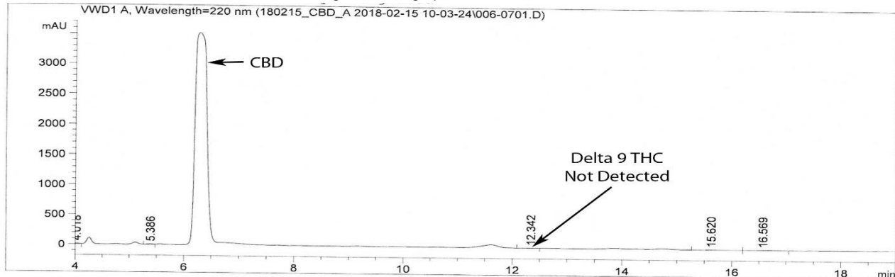
Testing Chromatograph for Batch 20816207
